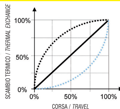
CURVA CARATTERISTICA INSTALLATA CHARACTERISTIC CURVE INSTALLED
